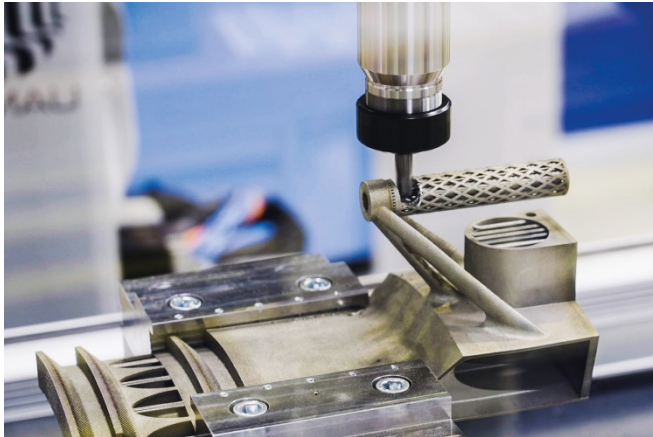
Image 4: Automatic, component-specific post-processing using a robot with subsequent verification by means of 3D scanning at Fraunhofer IWU in Chemnitz. © Fraunhofer.
